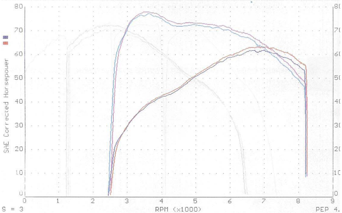
As measured on DYNJET'S MODEL 150 DYNAMOMETER
